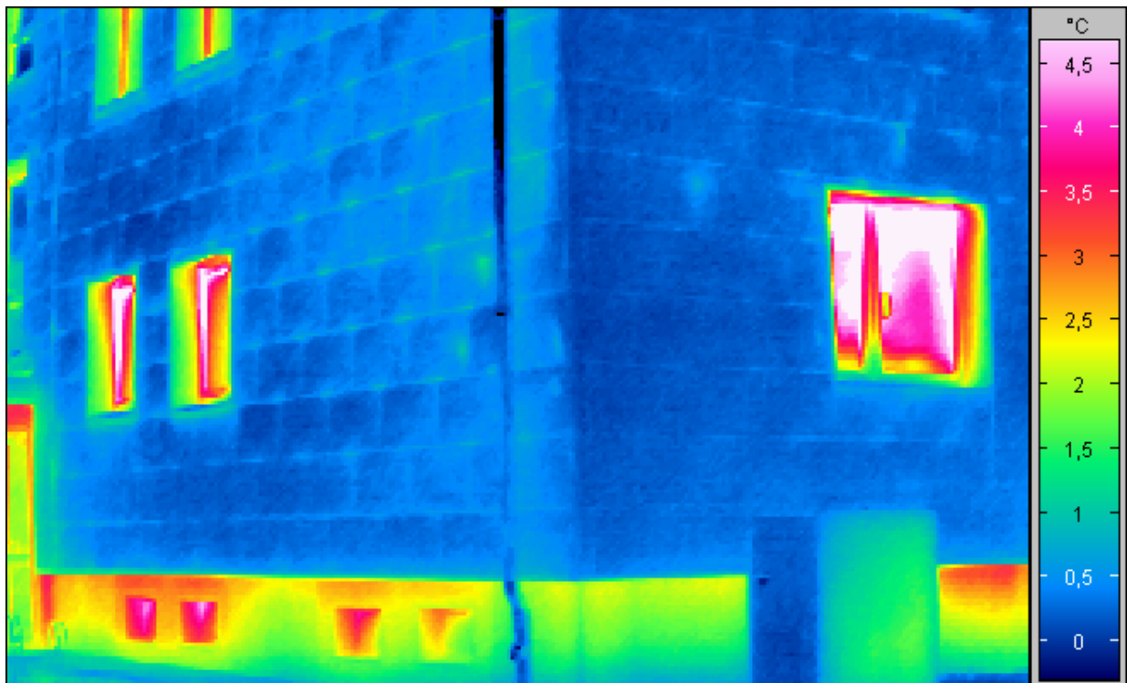
Building after reconstruction. Further existing lacks: poorly windows and no insulation of the basement
