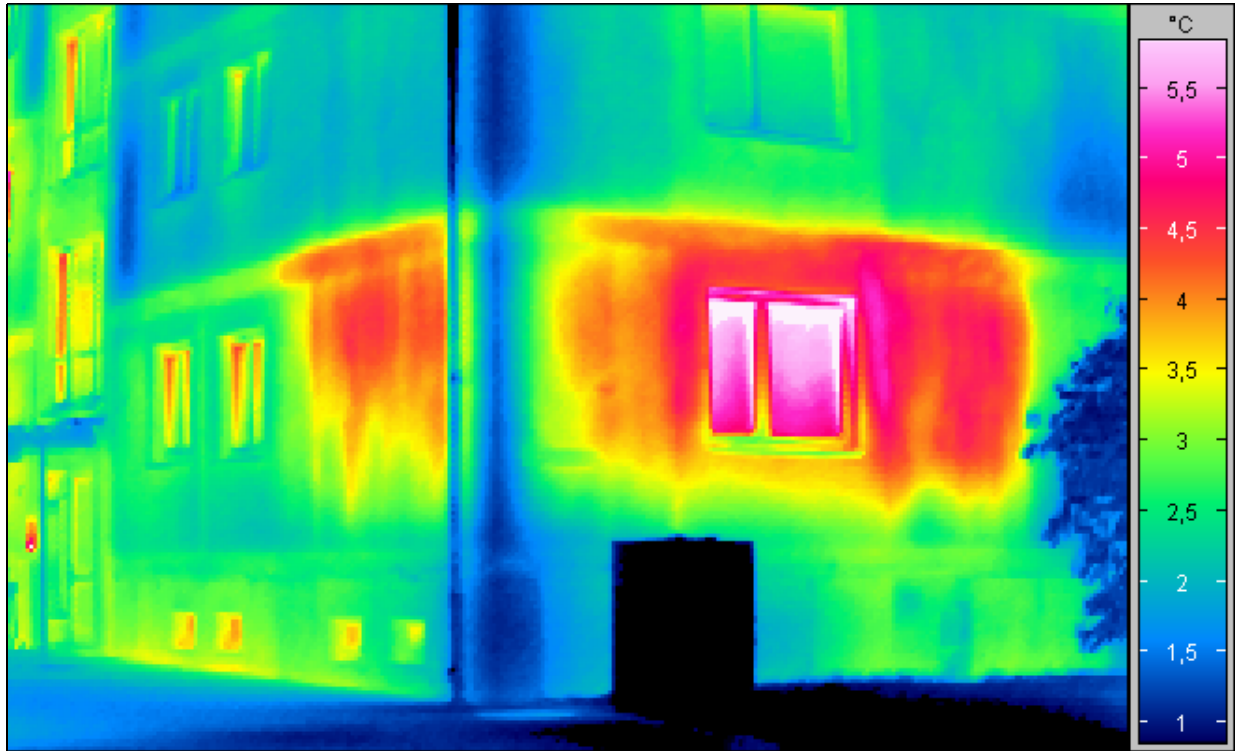
Insulation defects before reconstruction
